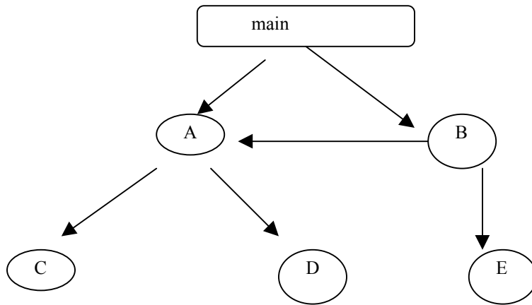
Figure 5.4 The graph of the desirable calls in the program in Figure 5.1
