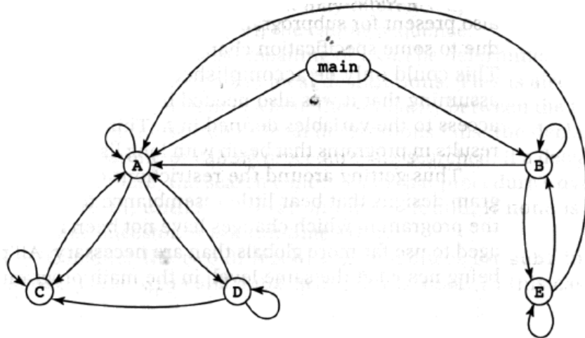
Figure 5.3 The potential call graph of the program in Figure 5.1
